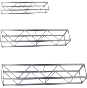
Straight section available in 9 lengths: 250, 300, 500, 750, 1000, 1250, 1500, 1750 & 2000mm (add UT-S before each length for the code)
