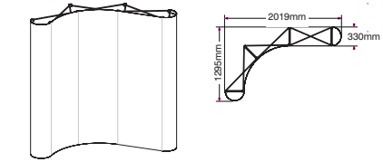
2.4m "L Shaped Pop-Up" exhibit kit
