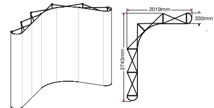
3m large "L Shaped Pop-Up" exhibit kit
