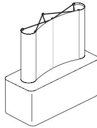
1.83m tabletop kit footprint dimensions: 1508mm h x 1854mm w x 489mm d
