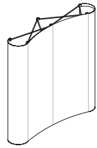
1.83m full height slim-line display system footprint dimensions: 2225mm h x 1930mm w x 485mm d
