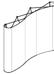
2.4m serpentine full height display system footprint dimensions: 2224mm h x 2273mm w x 495mm d
