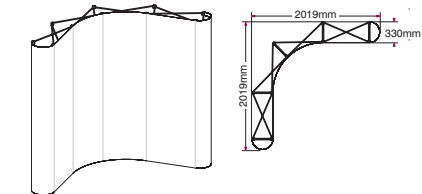
3m small "L Shaped Pop-Up" exhibit kit
