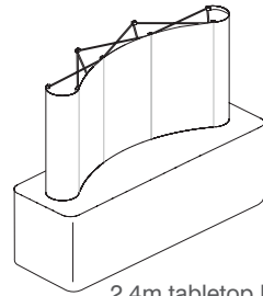
2.4m tabletop kit footprint dimensions: 1495mm h x 2540mm w x 685mm d
